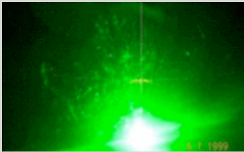
Glare from a legal 5 milliwatt laser pointer located 1200 feet from an aircraft. The runway cannot be seen when the laser is on the cockpit window.
